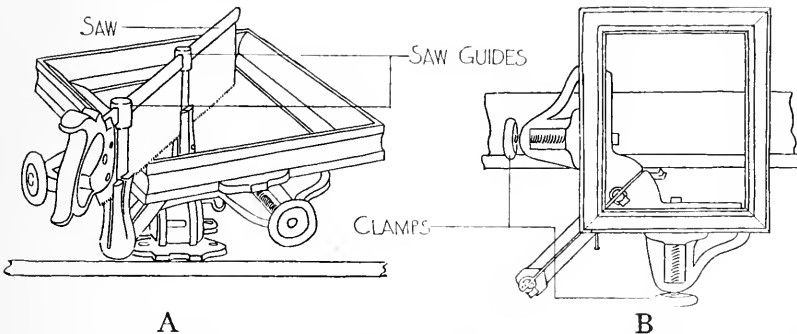
FIG. 215. PICTURE FRAME MITER BOX AND NAILING CLAMP.
